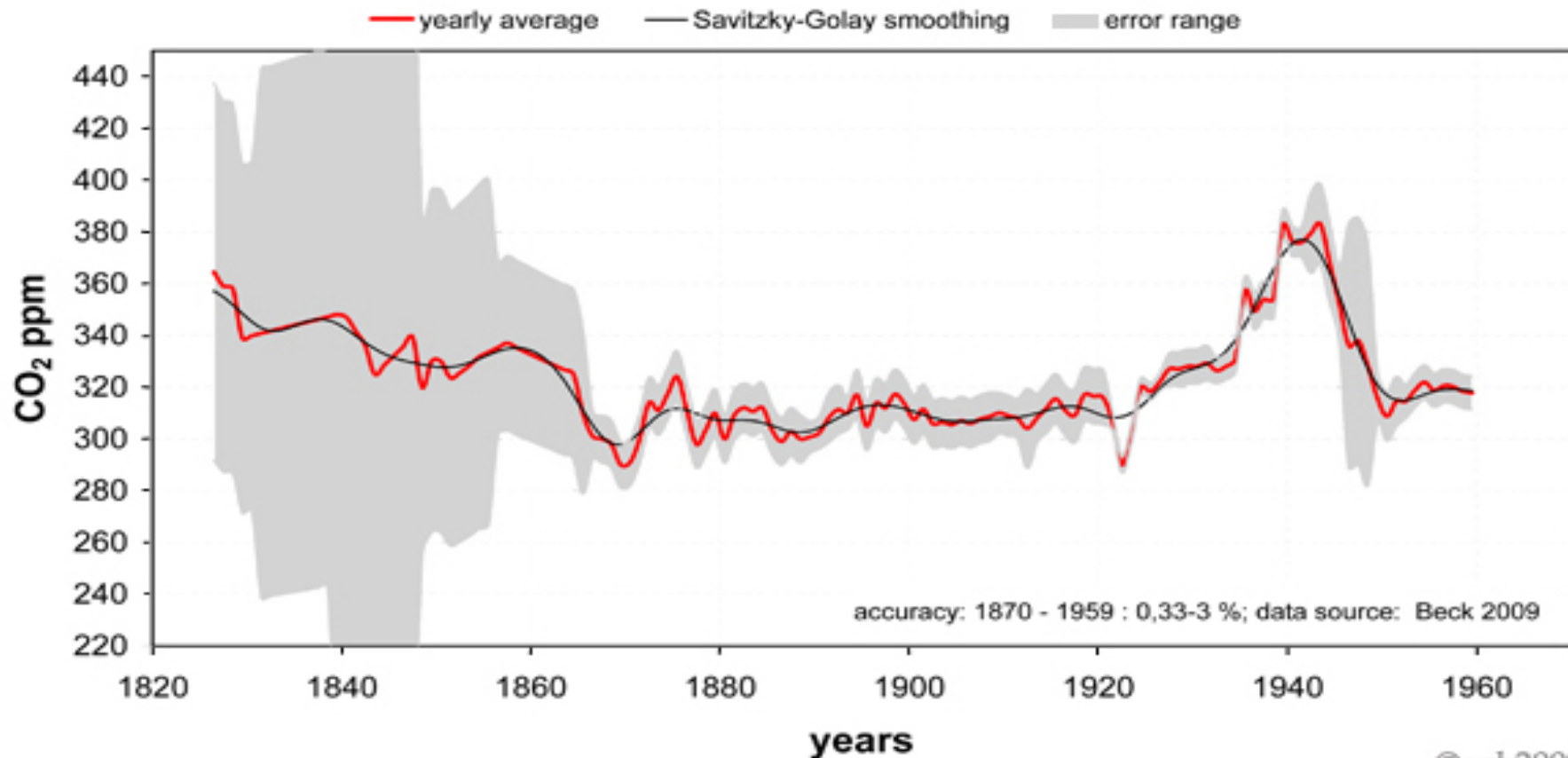
Atmospheric CO 2 Background 1826-1960
