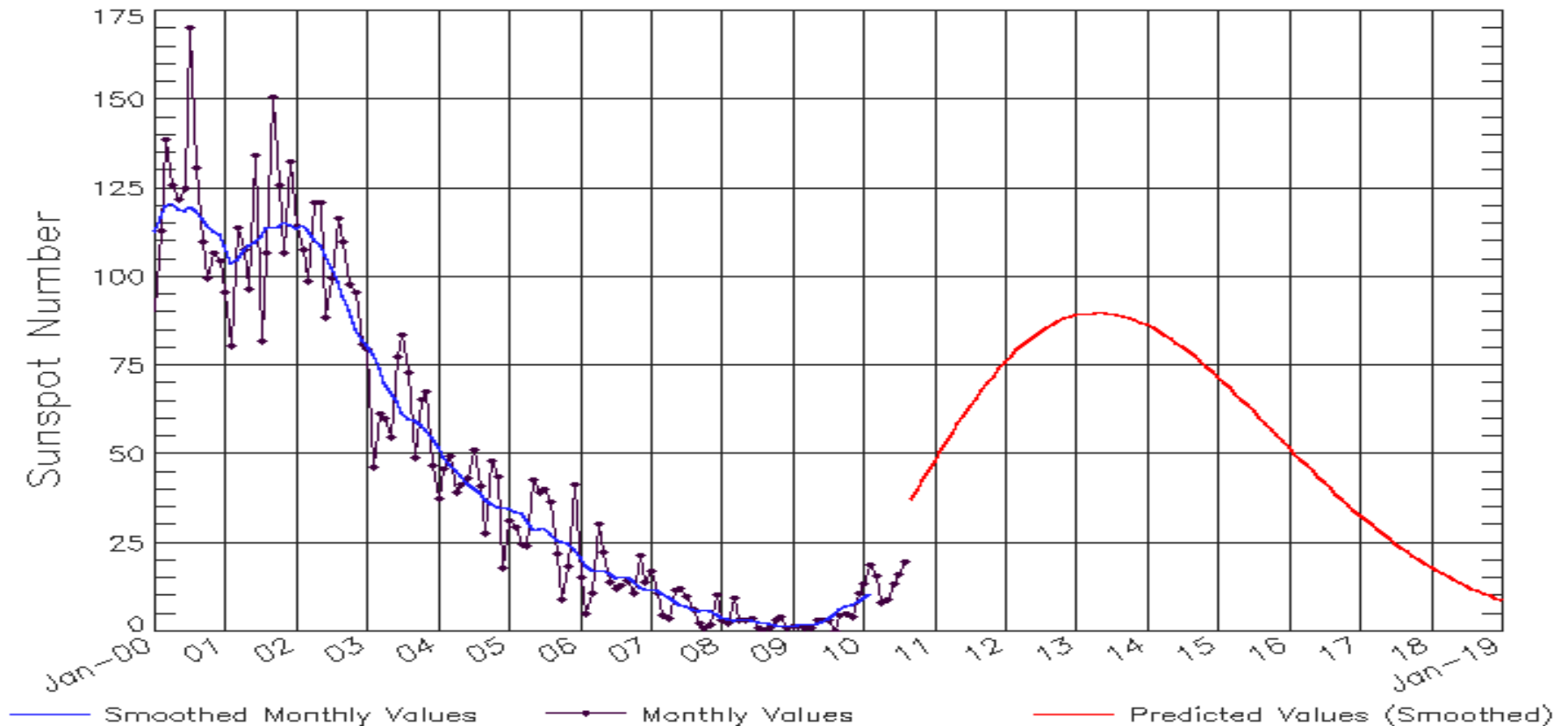
ISES Solar Cycle Sunspot Number Progression Observed data through Aug 2010
