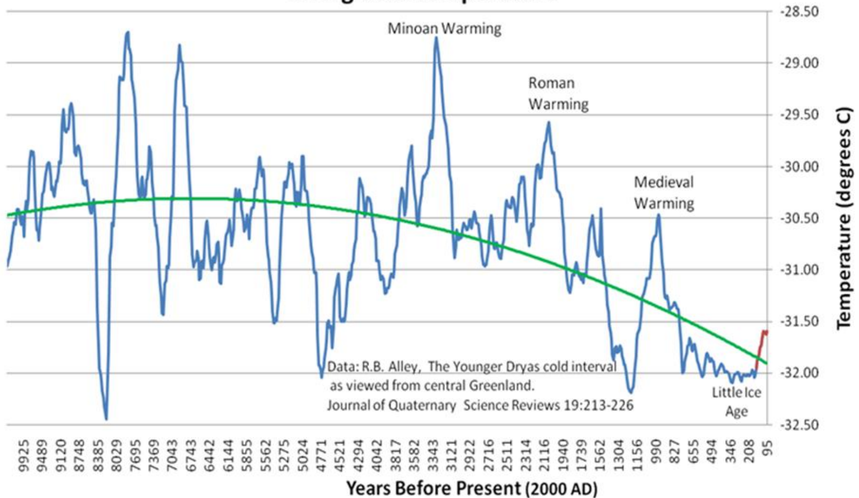
Greenland GISP2 Ice Core - Last 10,000 Years Interglacial Temperature
