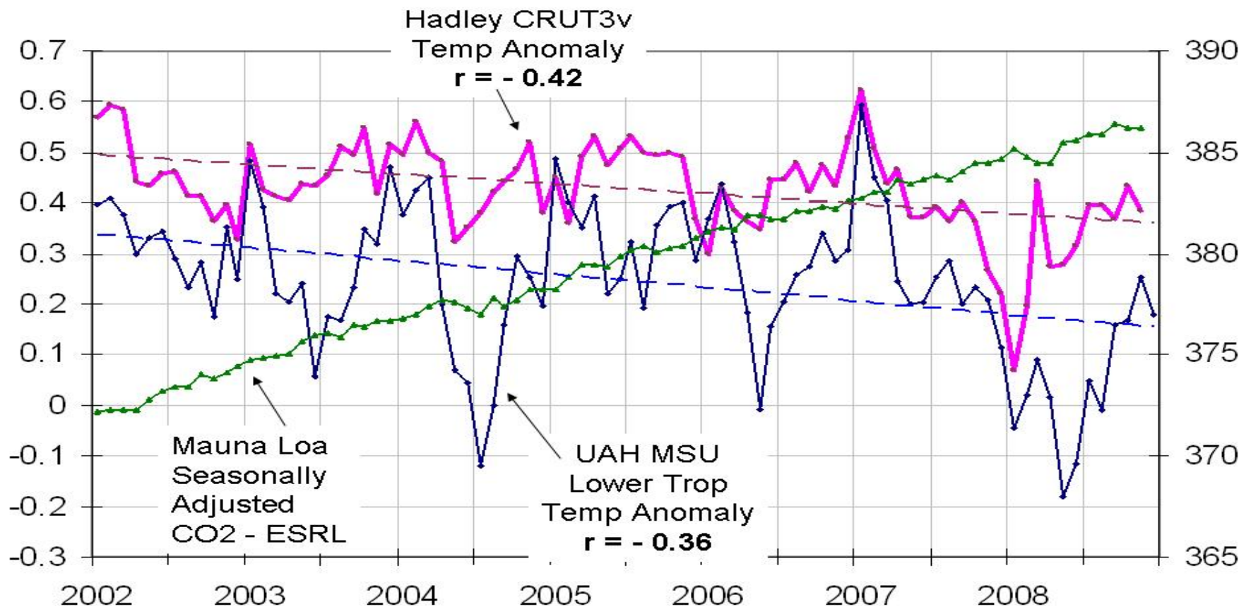
Hadley CRUT3v and UAH MSU vs CO2
